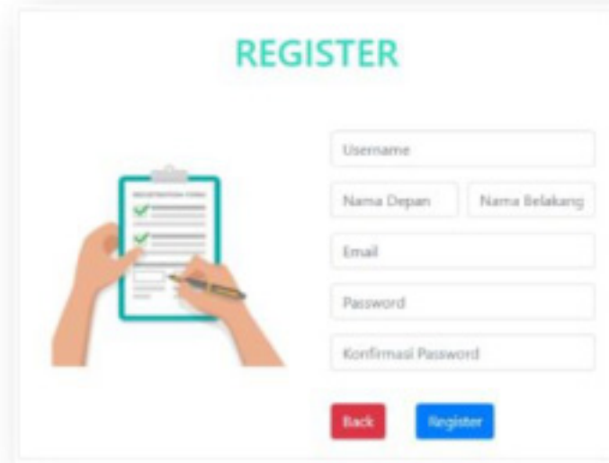
REGISTER
