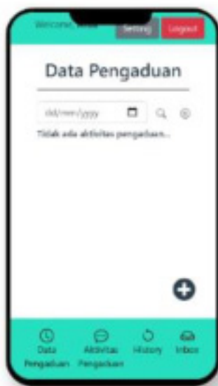
MOBILE RESPONSIVE
