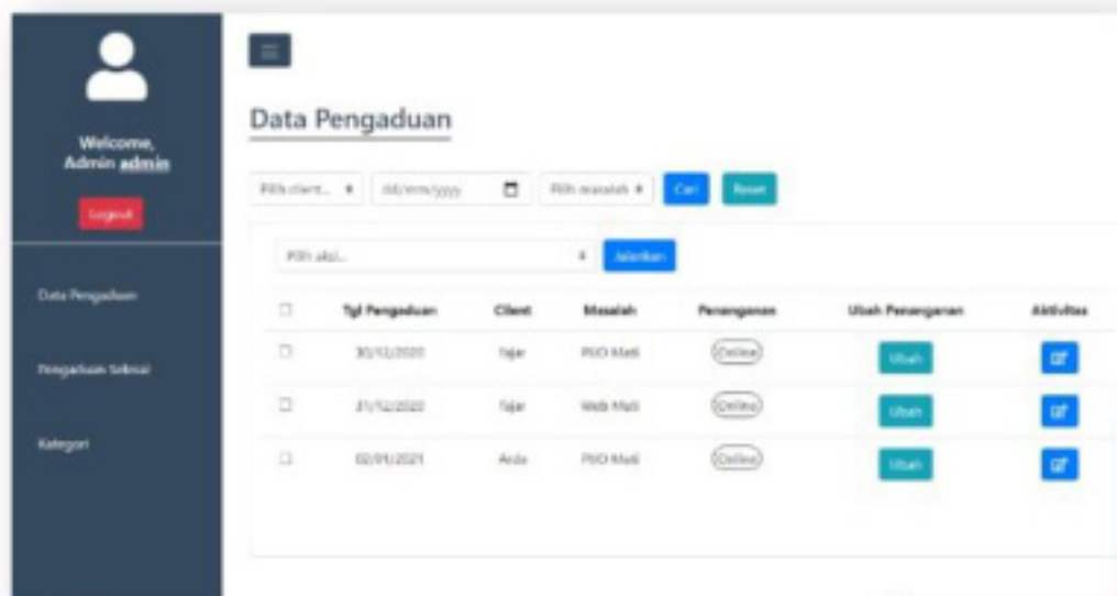
ADMIN INTERFACE
