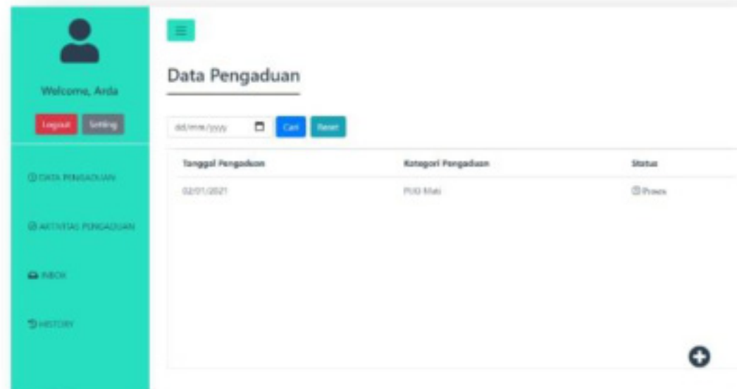
USER INTERFACE
